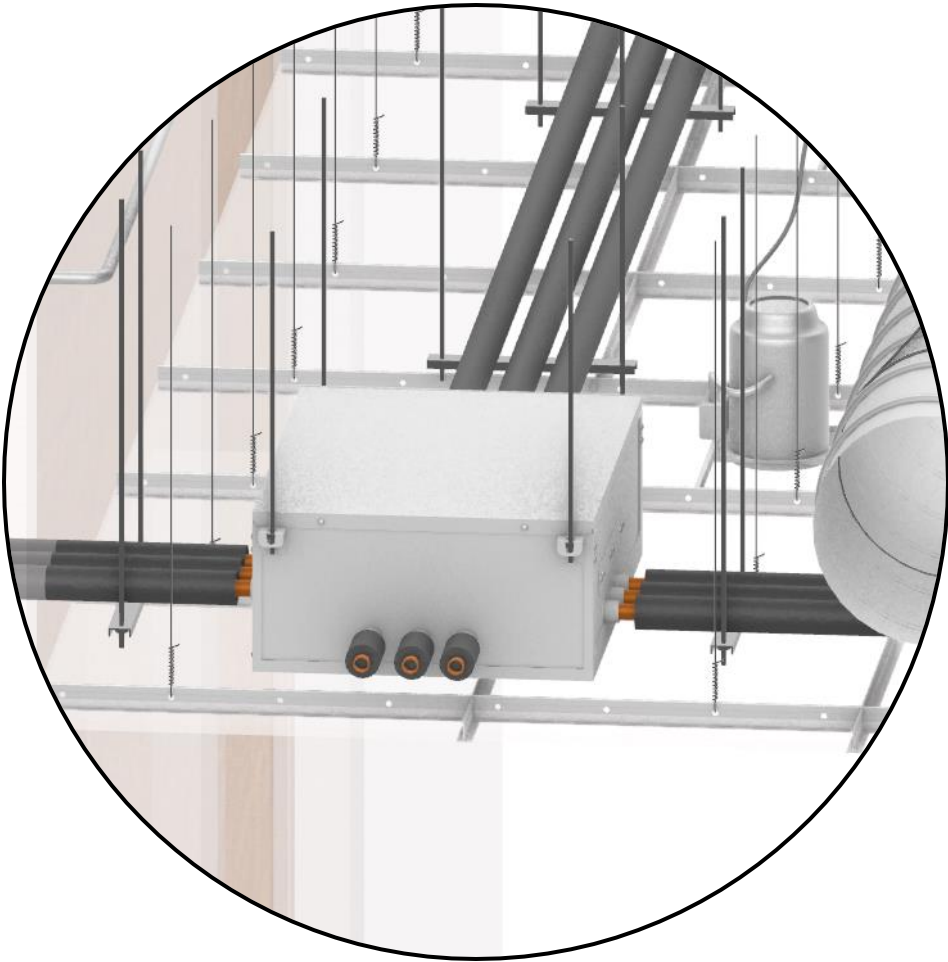
Branch Unit
