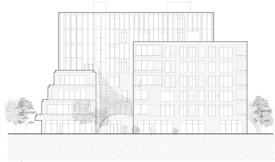
south elevation 152 shanley st
