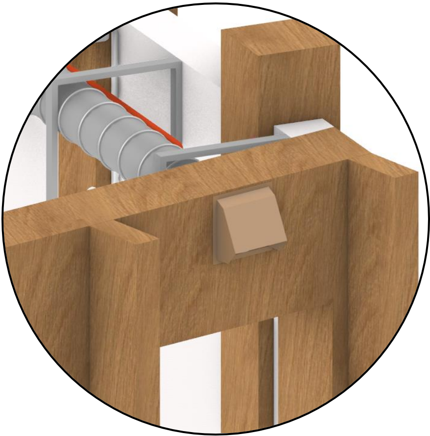
Exhaust
